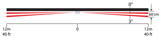
Wall (Top View)
