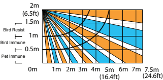
Side View (Sharp Mode Use Only)
